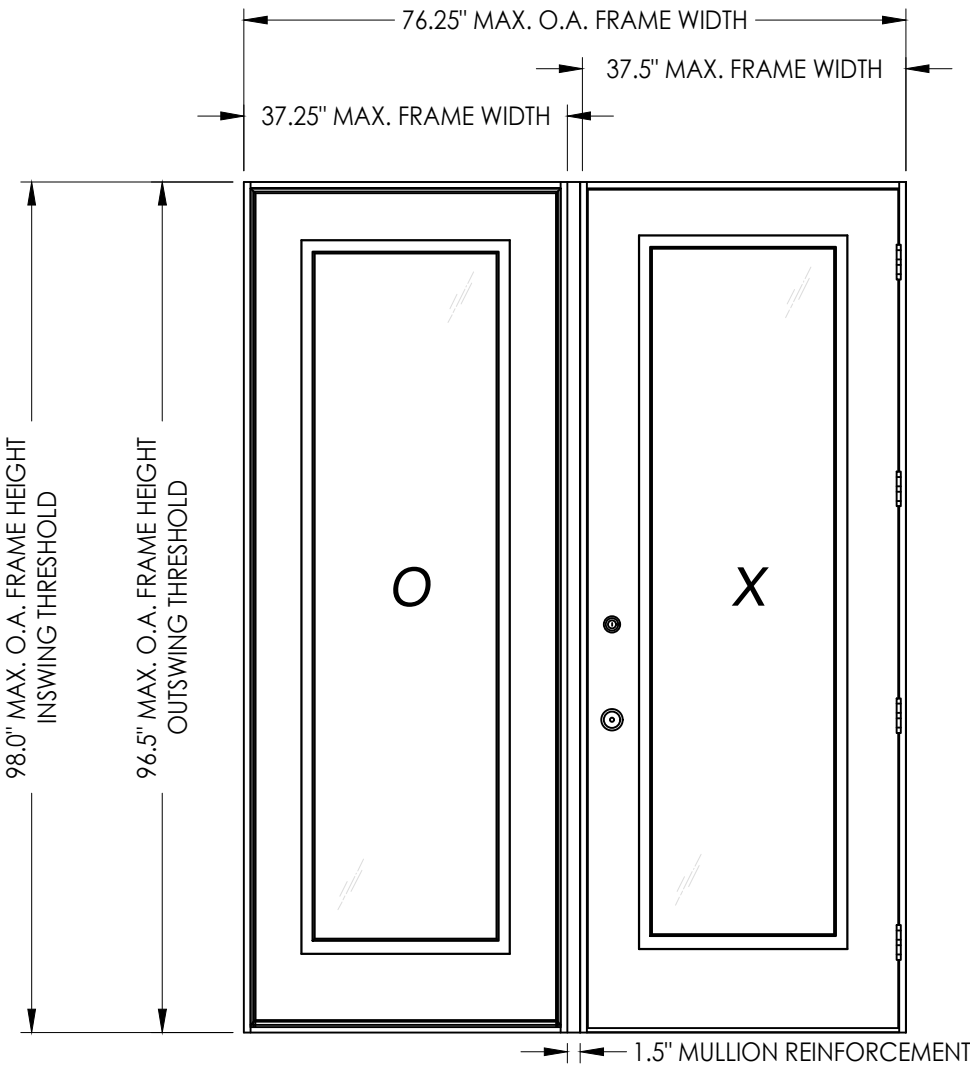
GLAZED SINGLE DOOR W/SIDELITE (OX configuration shown, XO also app'd)
